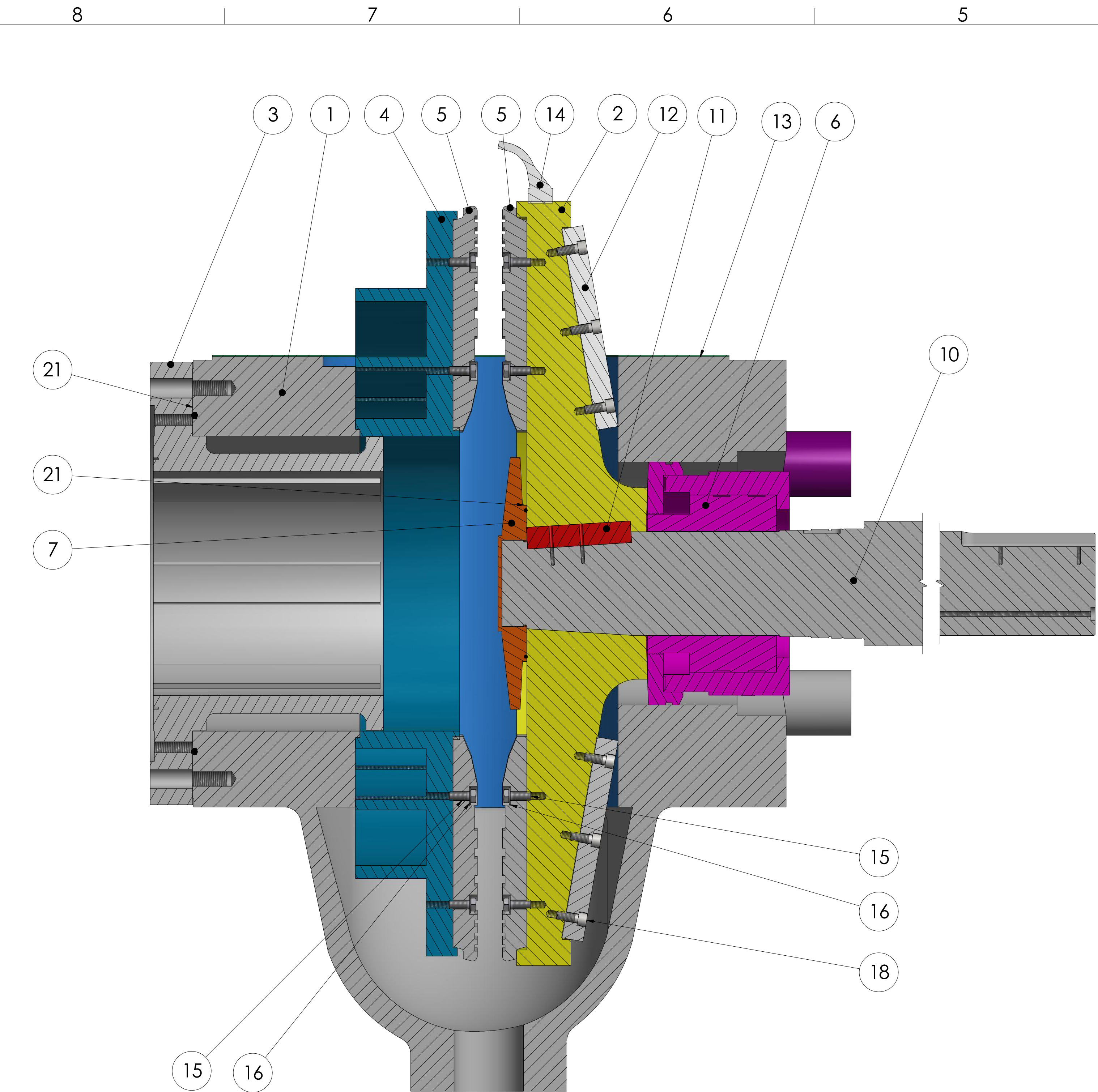
SECTION C-C
